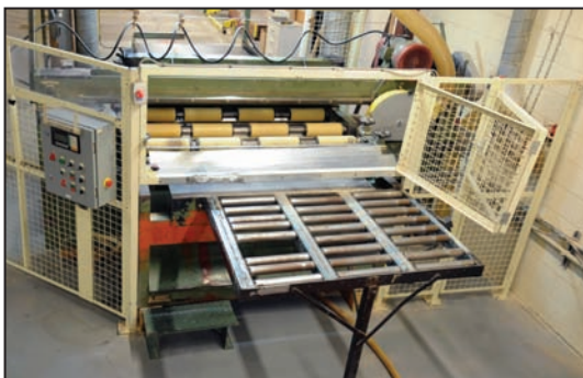
KIKUKAWA SRC 60 automatic panel sizing saw
