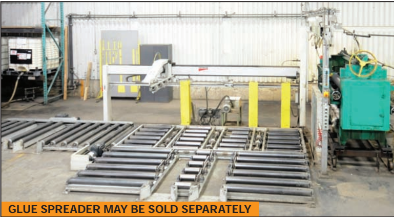
SP/160 pusher type panel feeder & BLACK BROTHERS 62" glue spreader
