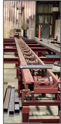
View of powered in-feed roller conveyor
