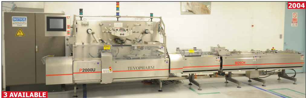
3 AVAILABLE BOSCH TEVOPHARM P2000U 3 station flow wrapper
