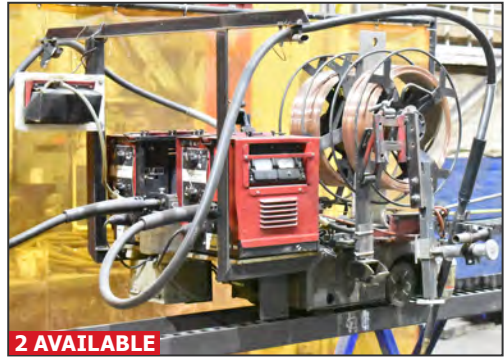
LINCOLN ELECTRIC LT-7 TRACTOR dual wire feed sub-arc tractor
